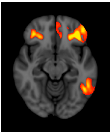
node 6 0.64
