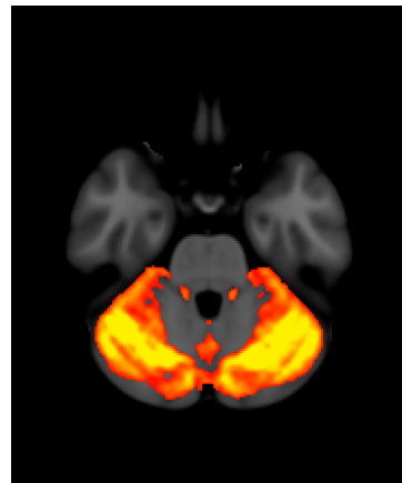
node 8 0.69
